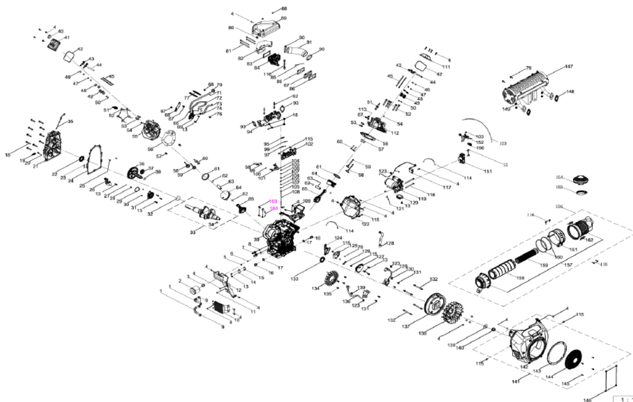
GB1000(1TA8QC10X) Part Illustrations
