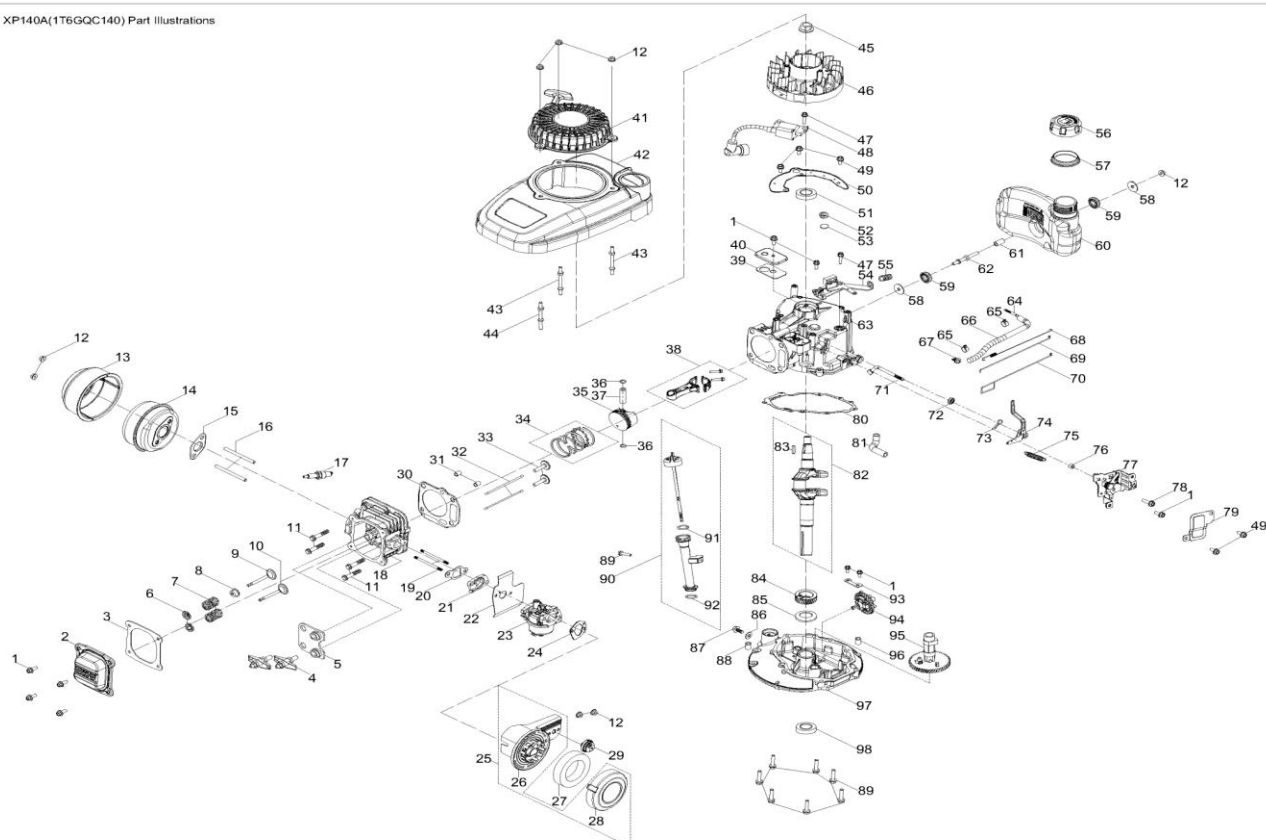
XP140A(1T6GQC140) Part Illustrations
